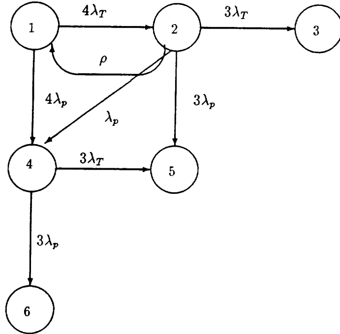
Figure 5: Reliability Model of a Quadruplex
