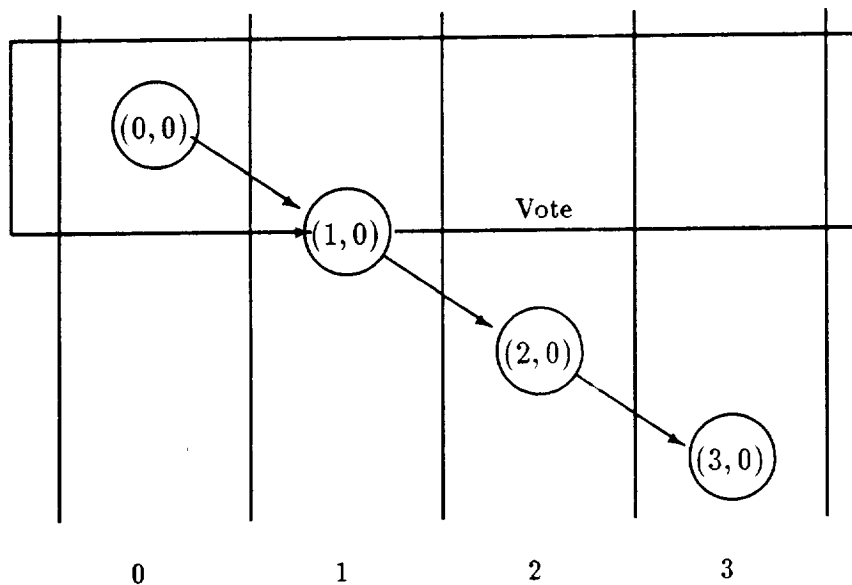
Figure 9: Example of task I/O graph.
